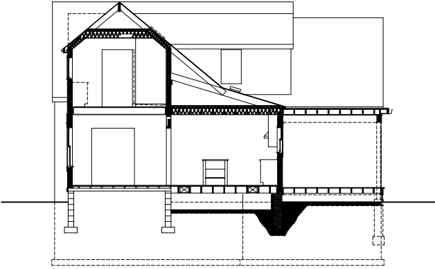
BUILDING SECTION
