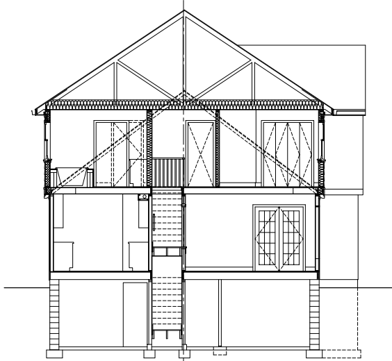
SOUTH-NORTH SECTION
