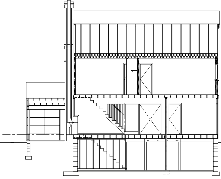
EAST-WEST SECTION
