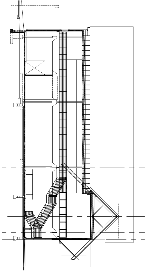
NORTH-SOUTH SECTION
