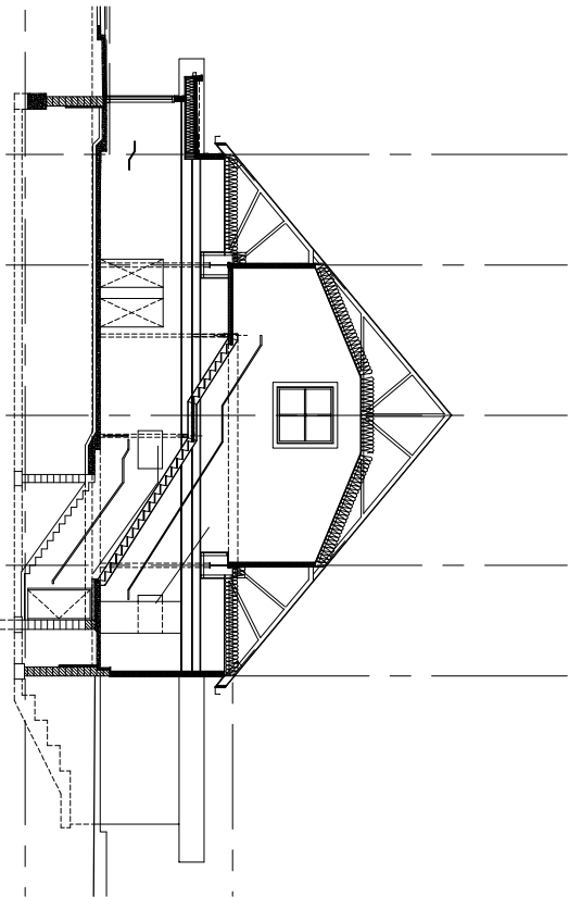
NORTH-SOUTH SECTION @ LINK
