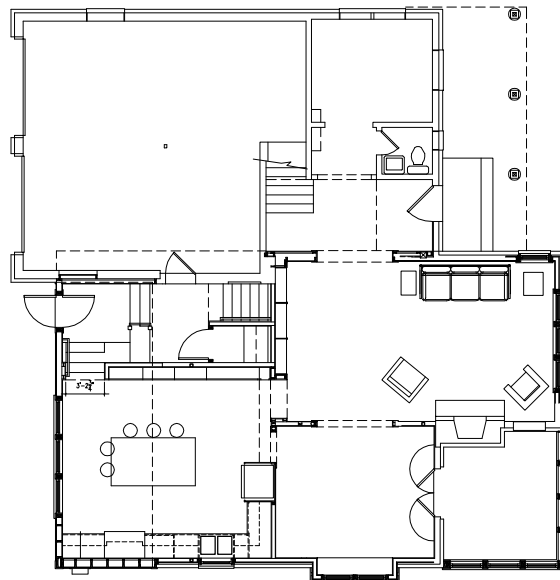
REMODELED MAIN FLOOR W/GARAGE & ADDITION
