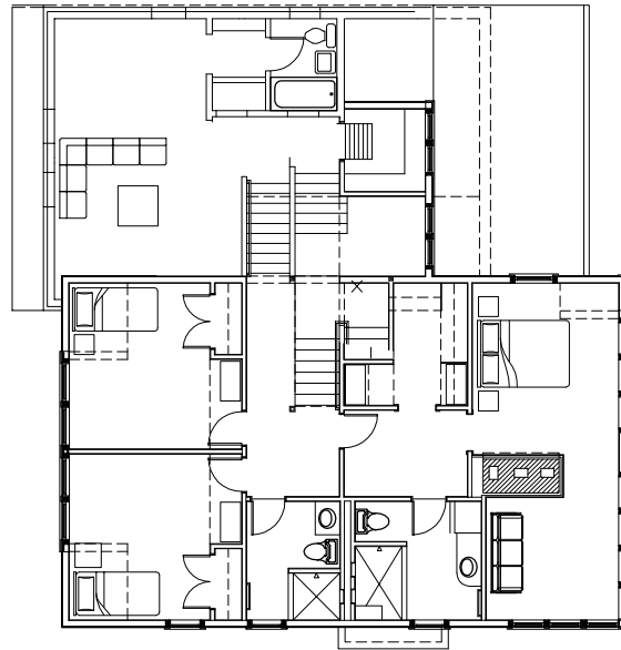
REMODELED 1/2 LEVEL W/ NEW SECOND FLOOR
