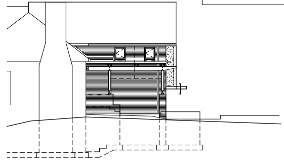
PARTIAL SOUTH ELEVATION
