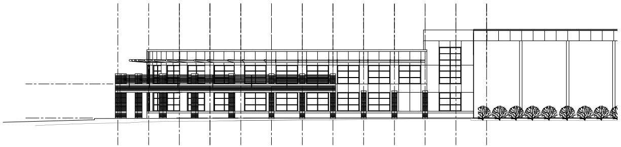
WEST ELEVATION
